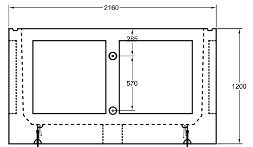
END PROFILE VIEW
