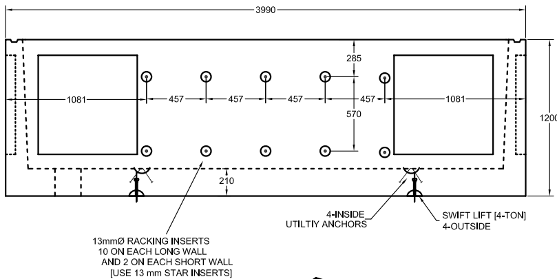
SIDE PROFILE VIEW
