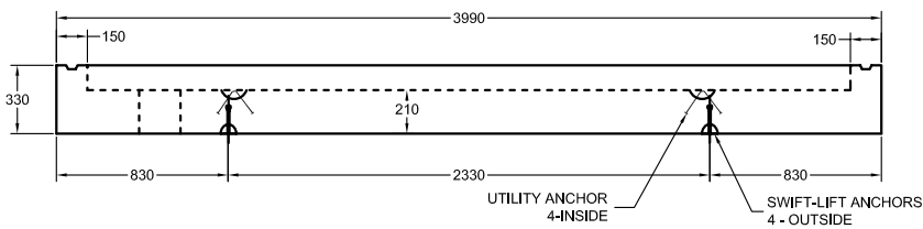
SIDE PROFILE VIEW
