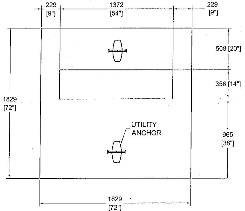
PLAN VIEW
